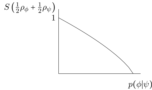
Figure 1.3: Entropy of a mixture of two pure states as a function of their Born rule.
